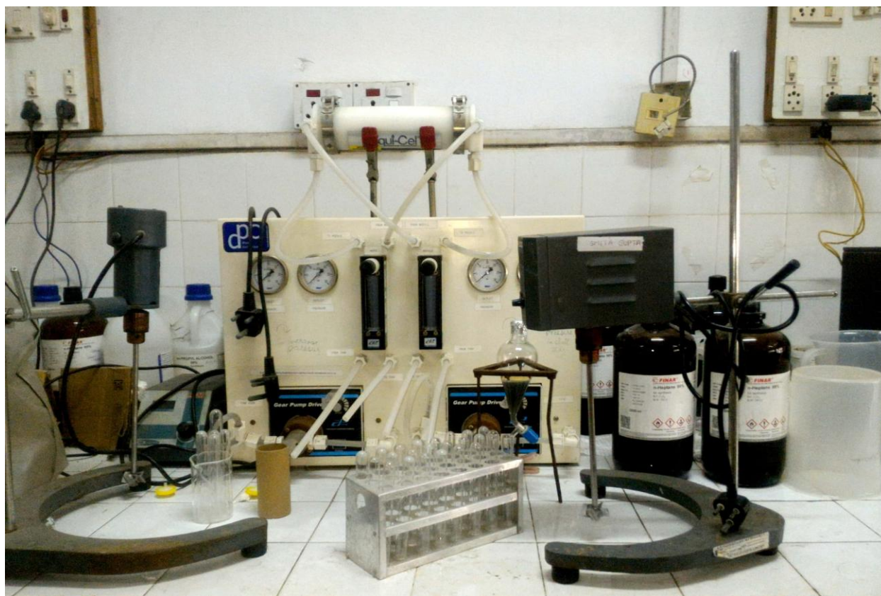
Set up 7: Liquid Membrane
